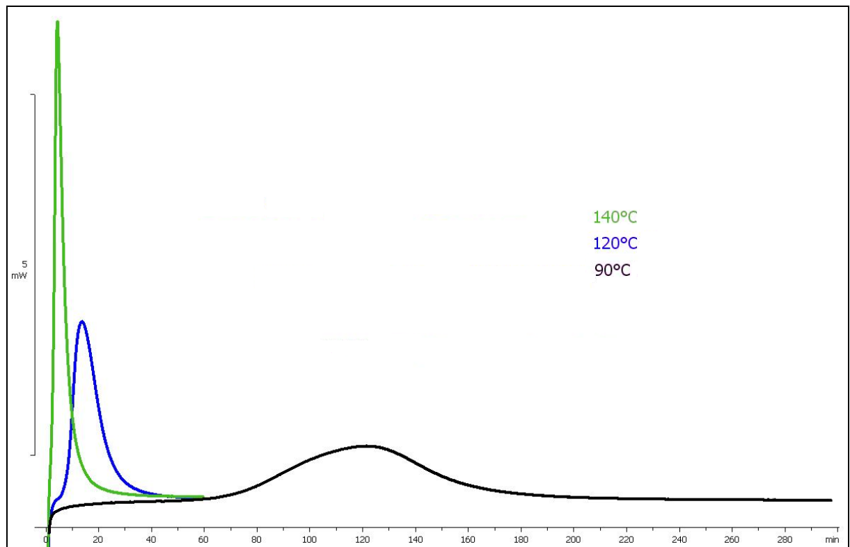
Fig. 2: Dependence of reaction rates on time at constant curing temperatures 90, 120 and 140 °C
