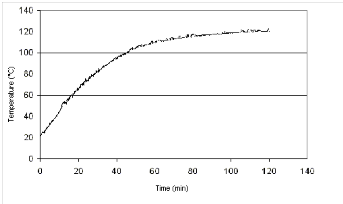
Fig. 3: Dependence of temperature inside the composition carbon fabric-Letoxit Foil 2.3mm thick. The composition was cured under vacuum in a steel mold at 120°C laid in a drying kiln.
